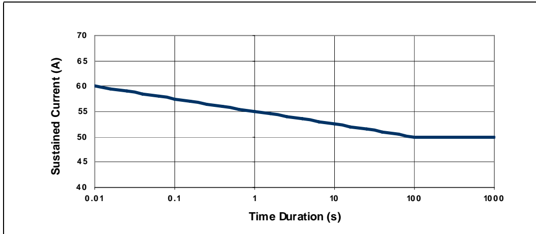
Figure 2-5. Quad-Core Intel® Xeon® Processor L5400 Series Load Current versus Time
